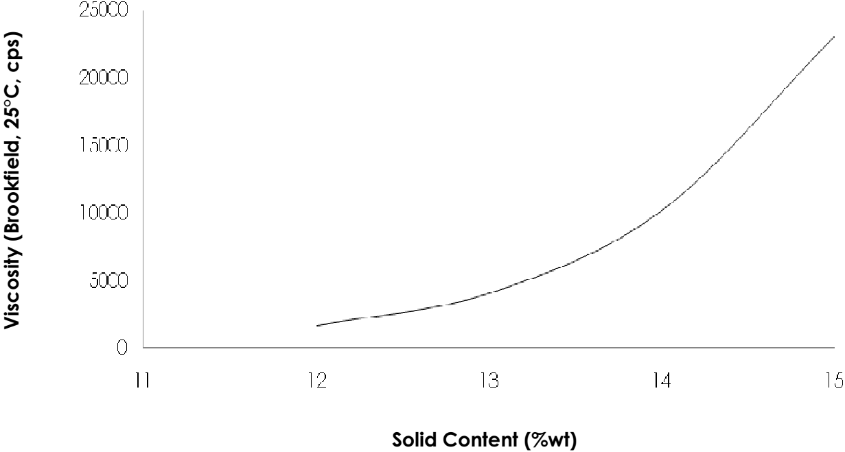
VISCOSITY Vs SOLIDS (pH 8.5)
